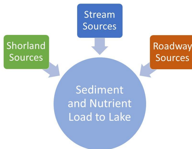
Figure 1: Conceptual diagram of primary water quality stressors on Lake Elmore.
