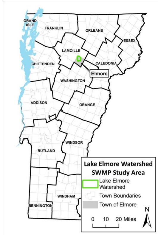
Figure 3: Lake Elmore watershed study area location map.
