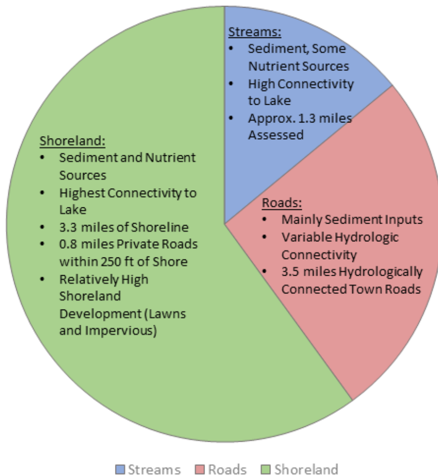
Figure 6: Relative contribution of sediment/nutrients to Lake Elmore from various sources.
